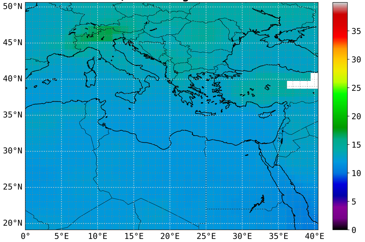
CO mean 3.0 km asl; scaling factor = 1e+08
