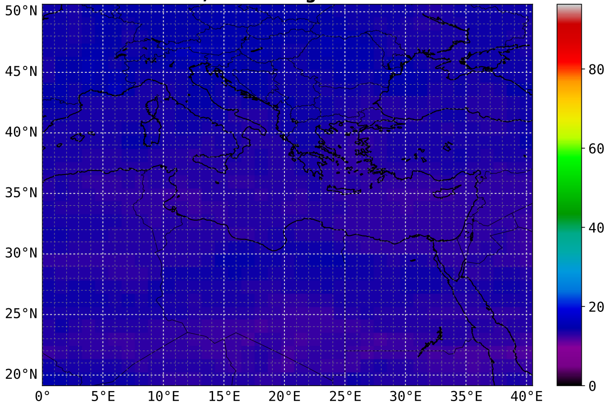
CO max 9.0 km asl; scaling factor = 1e+08
