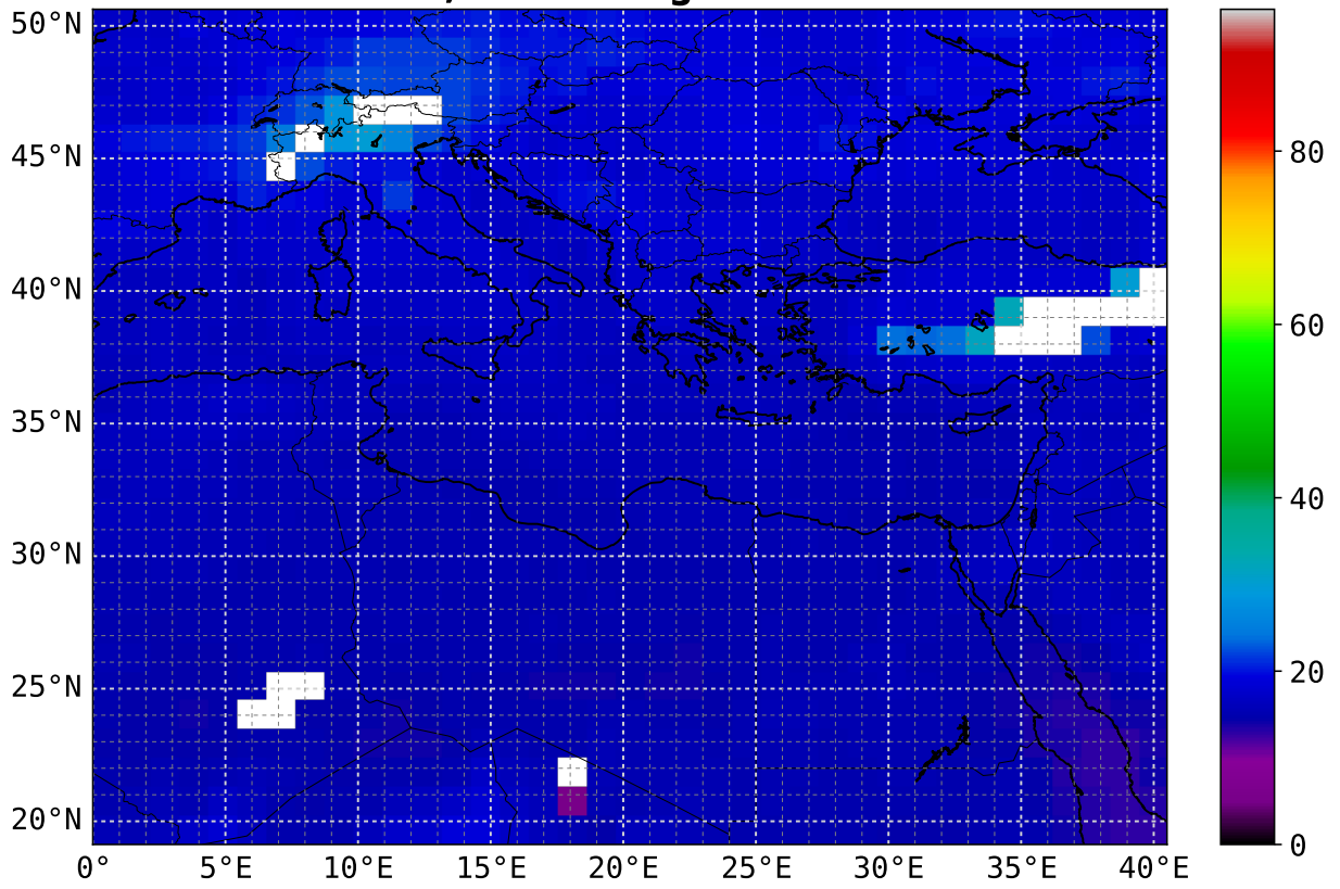
CO max 2.5 km asl; scaling factor = 1e+08
