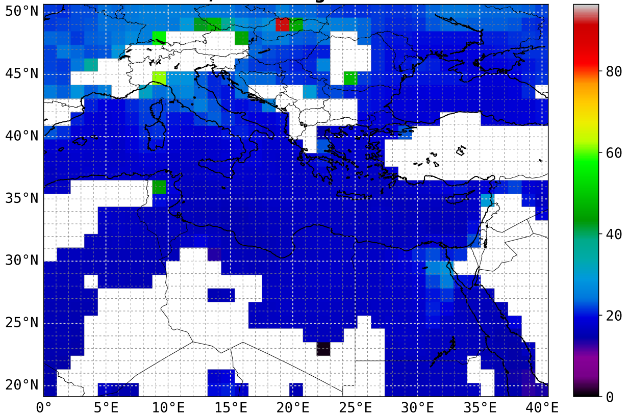
CO max 1.0 km asl; scaling factor = 1e+08
