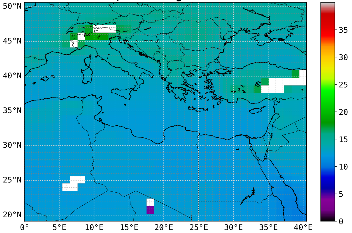
CO mean 2.5 km asl; scaling factor = 1e+08
