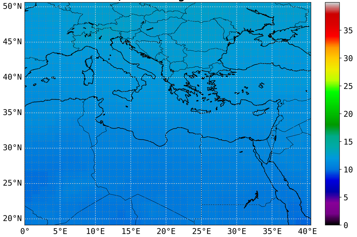
CO mean 6.5 km asl; scaling factor = 1e+08
