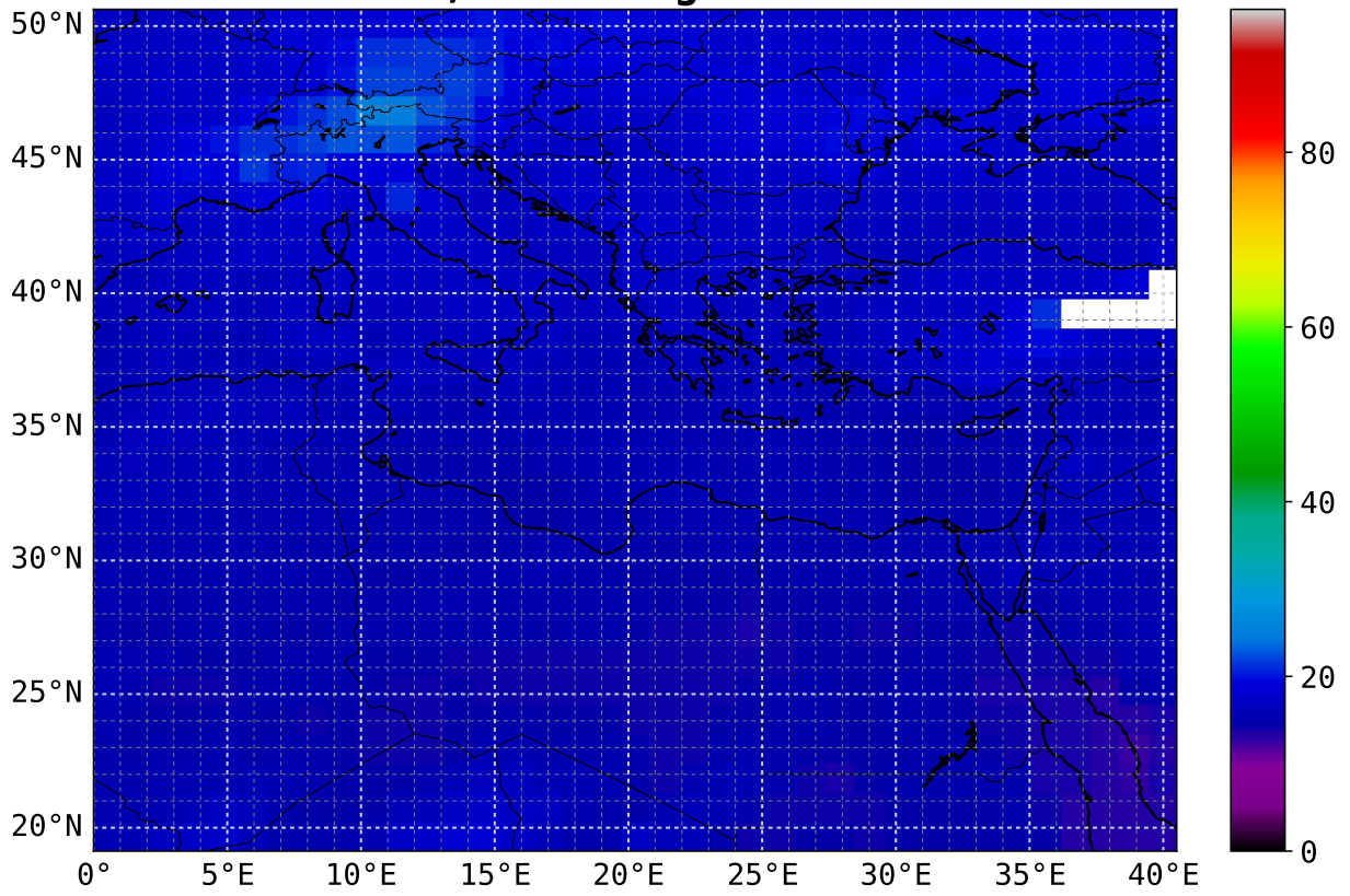
CO max 3.0 km asl; scaling factor = 1e+08
