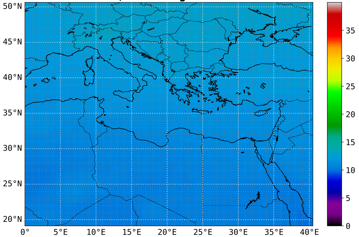
CO mean 6.0 km asl; scaling factor = 1e+08
