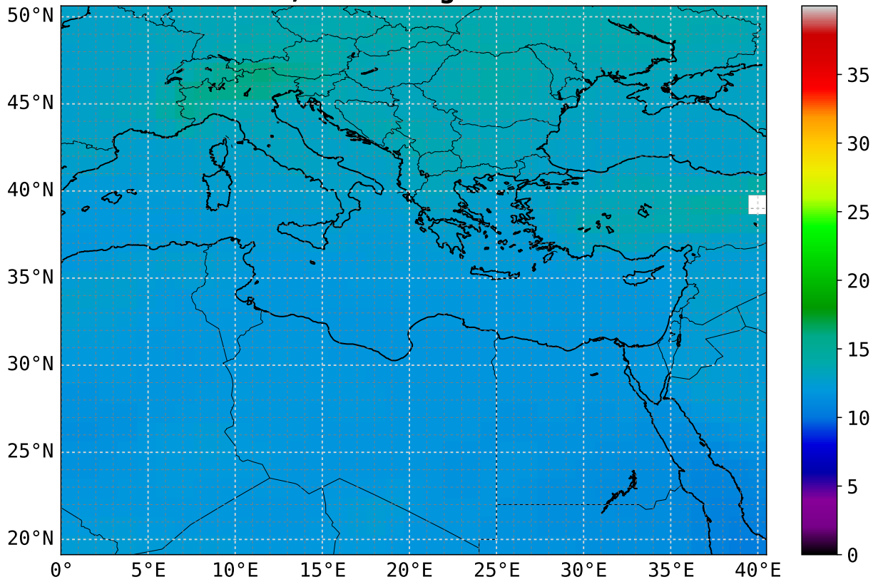
CO mean 3.5 km asl; scaling factor = 1e+08
