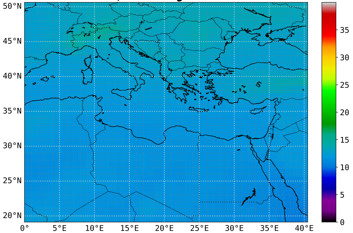
CO mean 4.0 km asl; scaling factor = 1e+08
