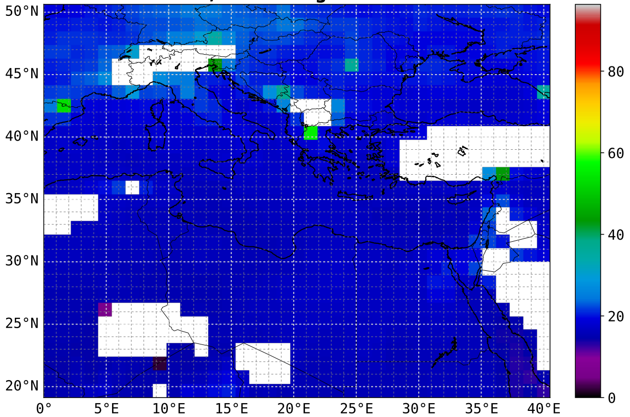
CO max 1.5 km asl; scaling factor = 1e+08
