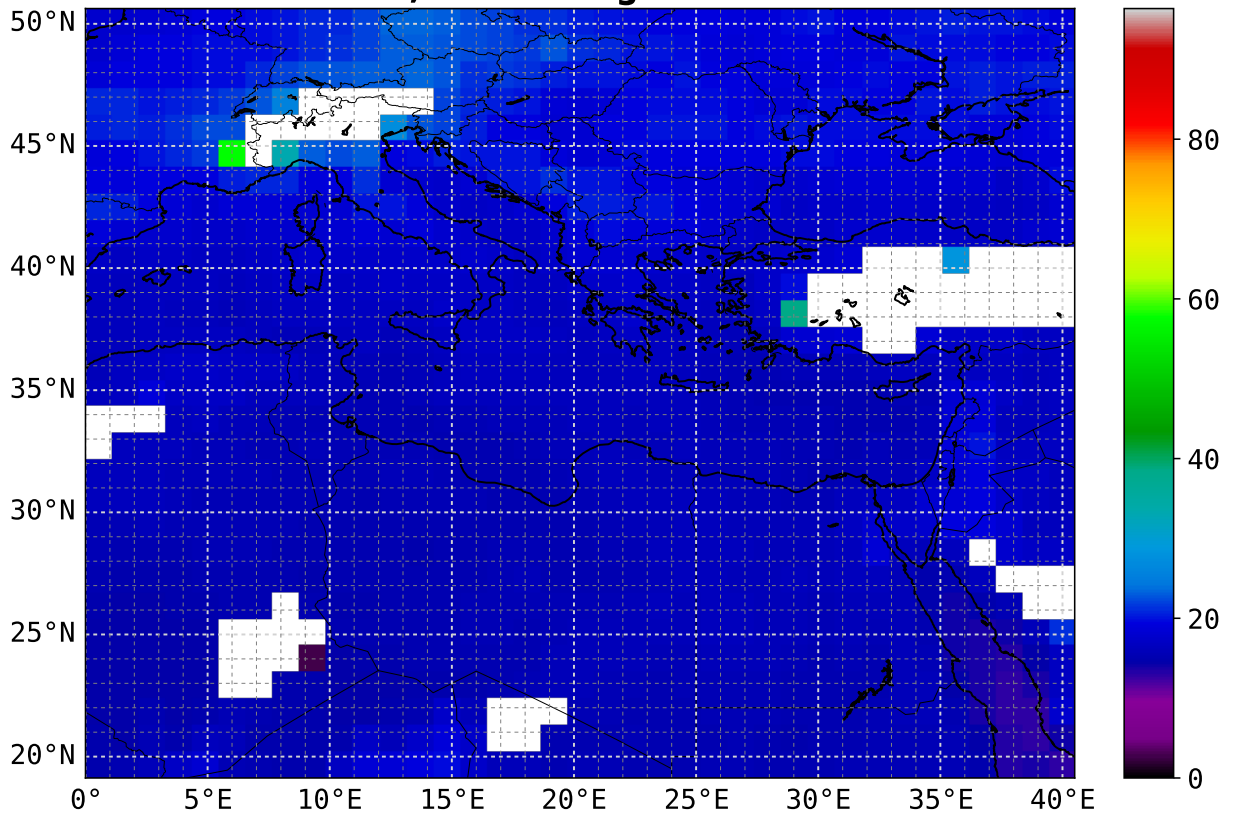
CO max 2.0 km asl; scaling factor = 1e+08
