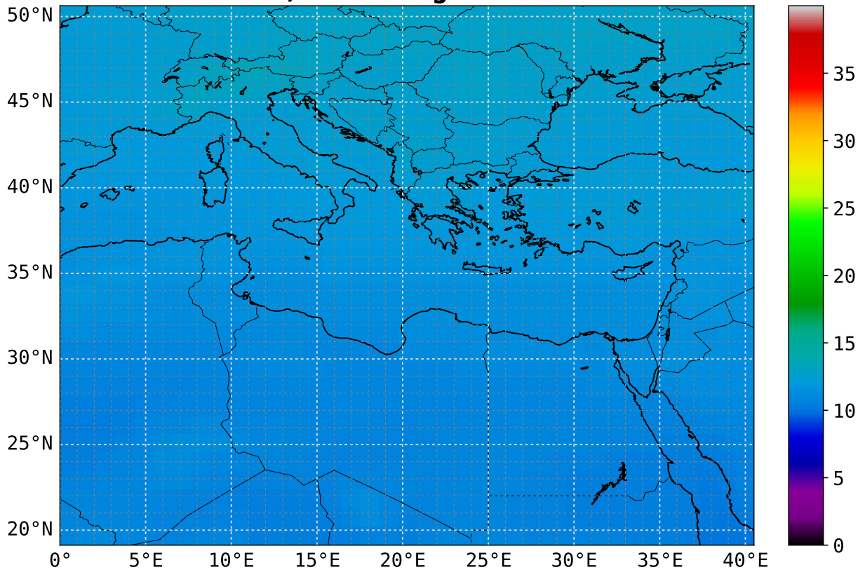
C0 mean 5.5 km asl; scaling factor = 1e+08
