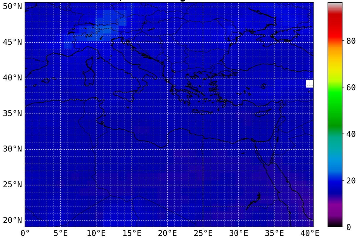
CO max 3.5 km asl; scaling factor = 1e+08
