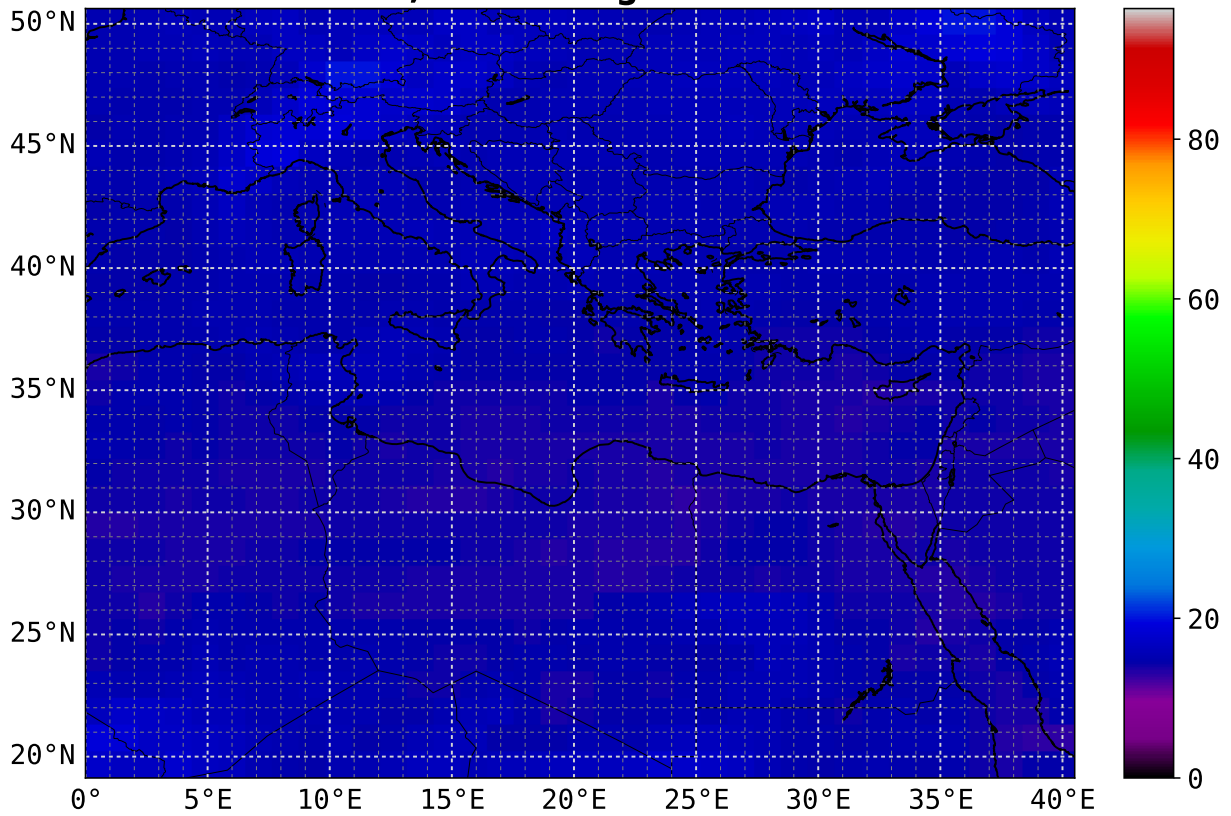
CO max 18 UTC 5.0 km asl; scaling factor = 1e+08
