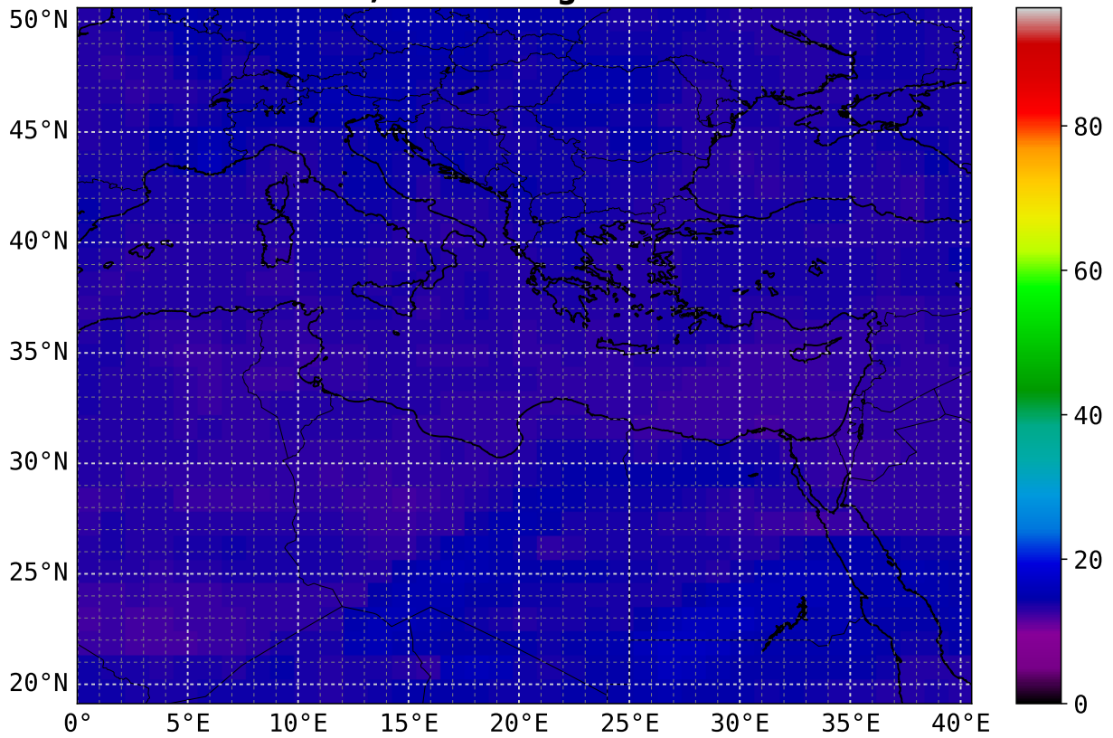
CO max 18 UTC 9.0 km asl; scaling factor = 1e+08
