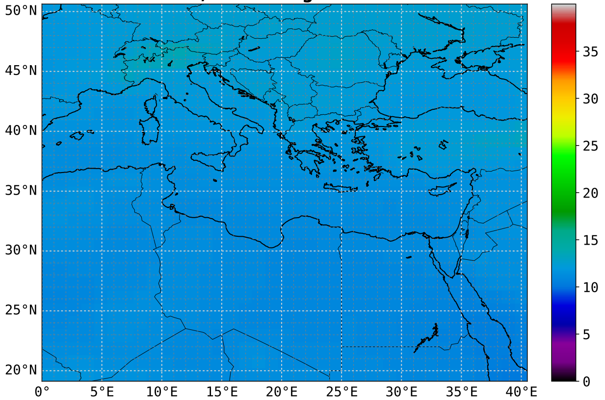
CO mean 18 UTC 4.0 km asl; scaling factor = 1e+08
