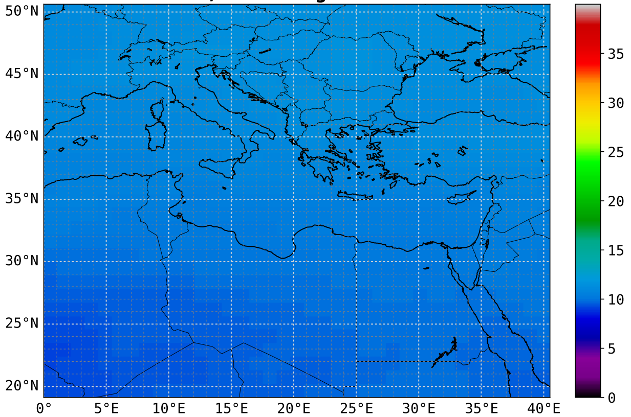
CO mean 18 UTC 8.0 km asl; scaling factor = 1e+08
