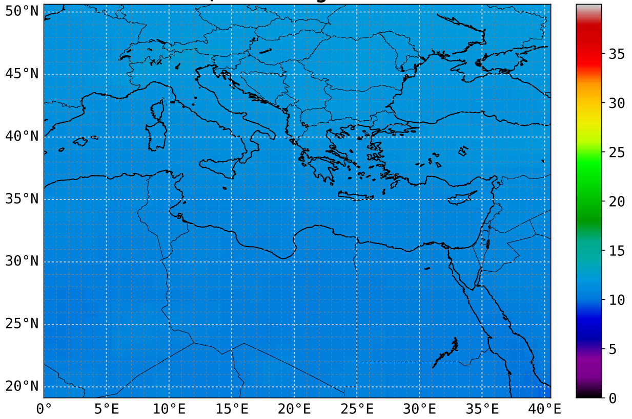
CO mean 18 UTC 5.5 km asl; scaling factor = 1e+08
