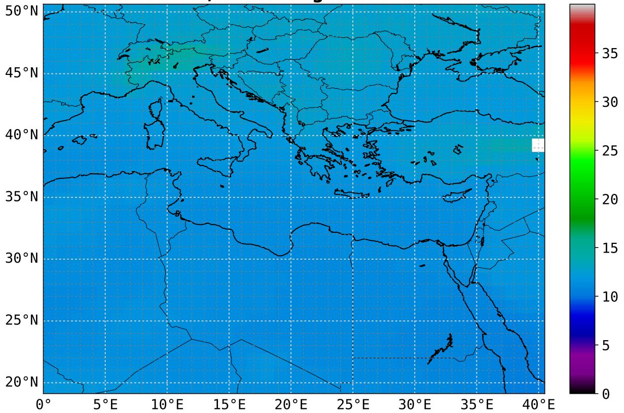
CO mean 18 UTC 3.5 km asl; scaling factor = 1e+08
