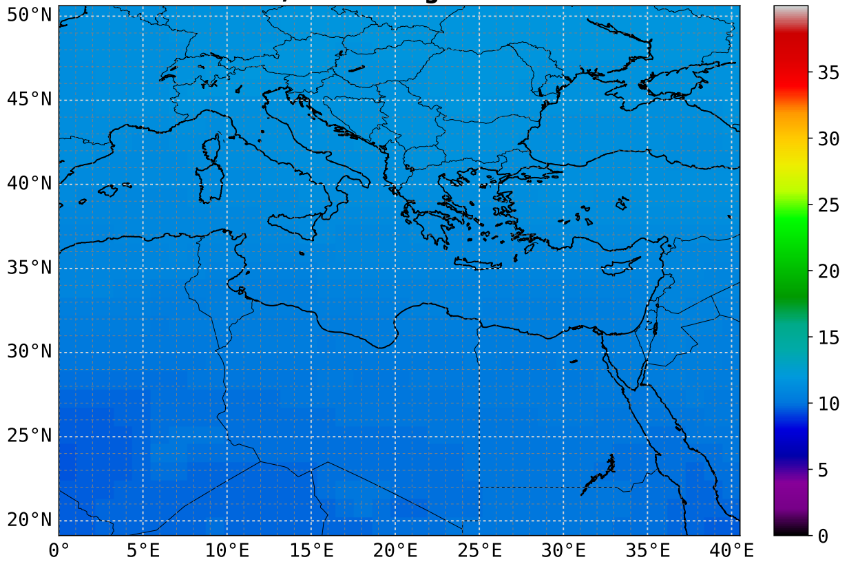
CO mean 18 UTC 7.0 km asl; scaling factor = 1e+08
