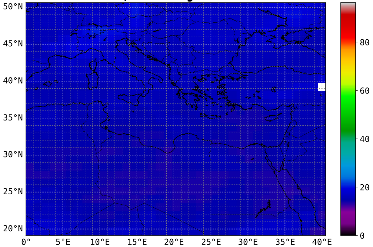
CO max 18 UTC 3.5 km asl; scaling factor = 1e+08
