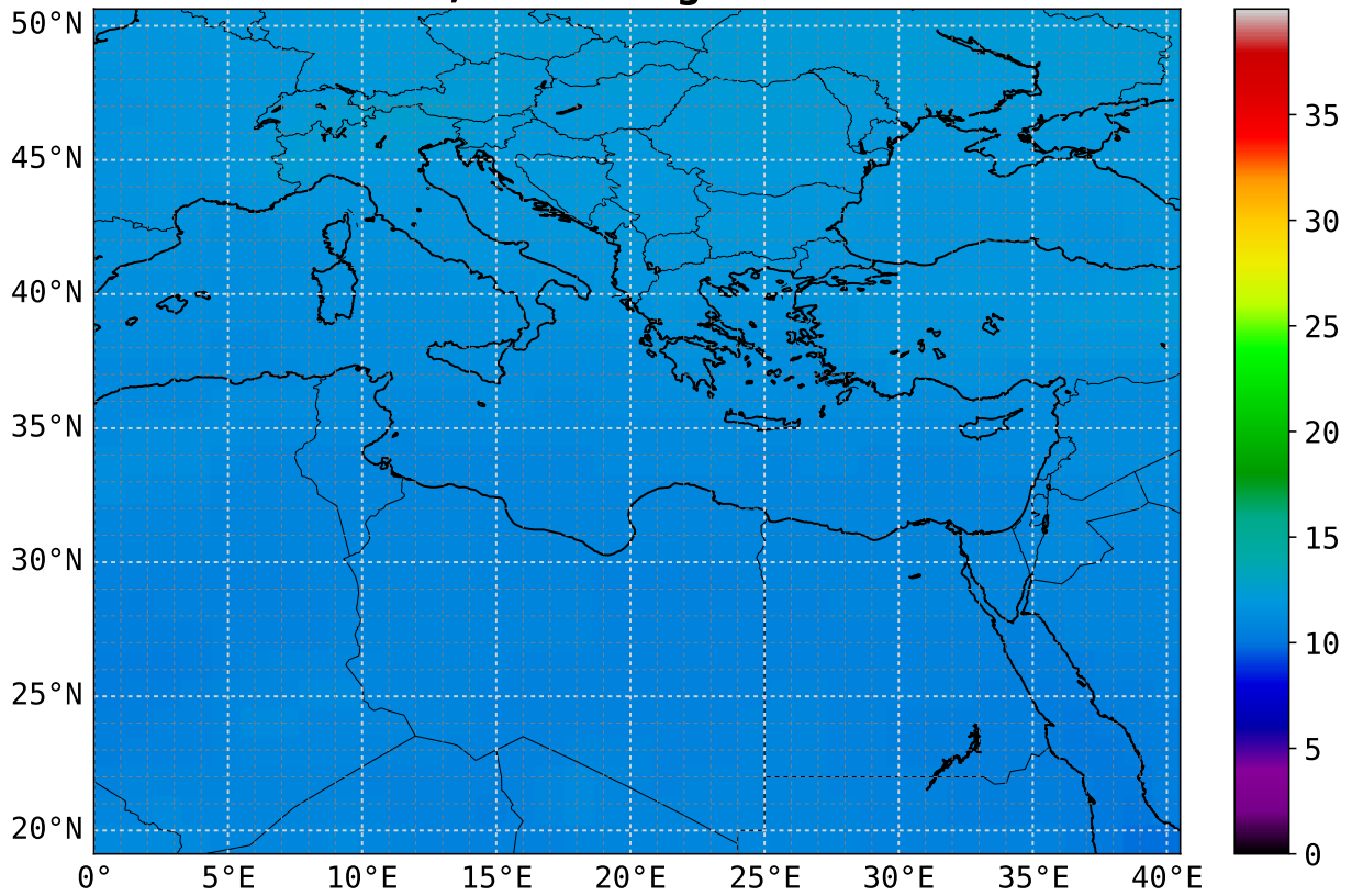
CO mean 18 UTC 5.0 km asl; scaling factor = 1e+08
