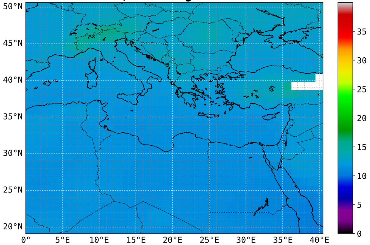
CO mean 18 UTC 3.0 km asl; scaling factor = 1e+08
