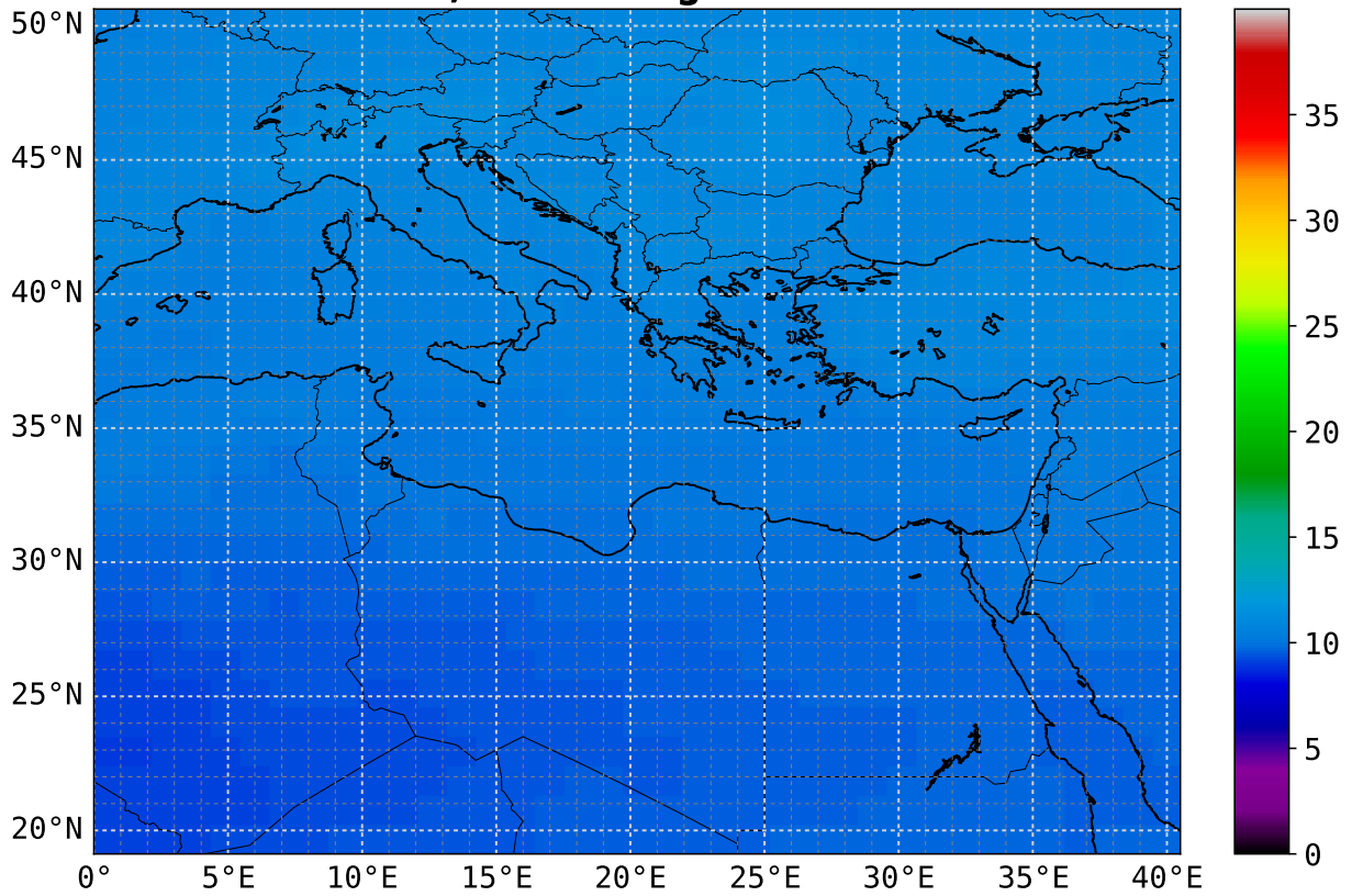
CO mean 18 UTC 9.0 km asl; scaling factor = 1e+08
