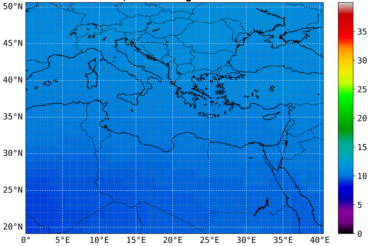
CO mean 18 UTC 8.5 km asl; scaling factor = 1e+08
