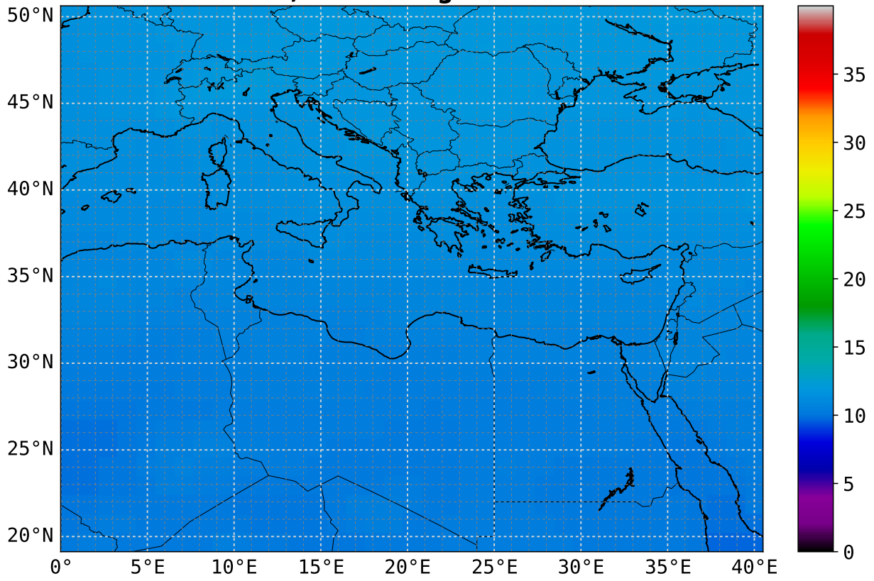
CO mean 18 UTC 6.0 km asl; scaling factor = 1e+08
