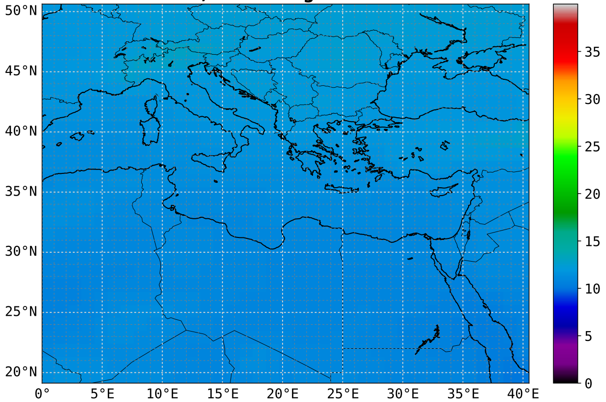
CO mean 18 UTC 4.5 km asl; scaling factor = 1e+08
