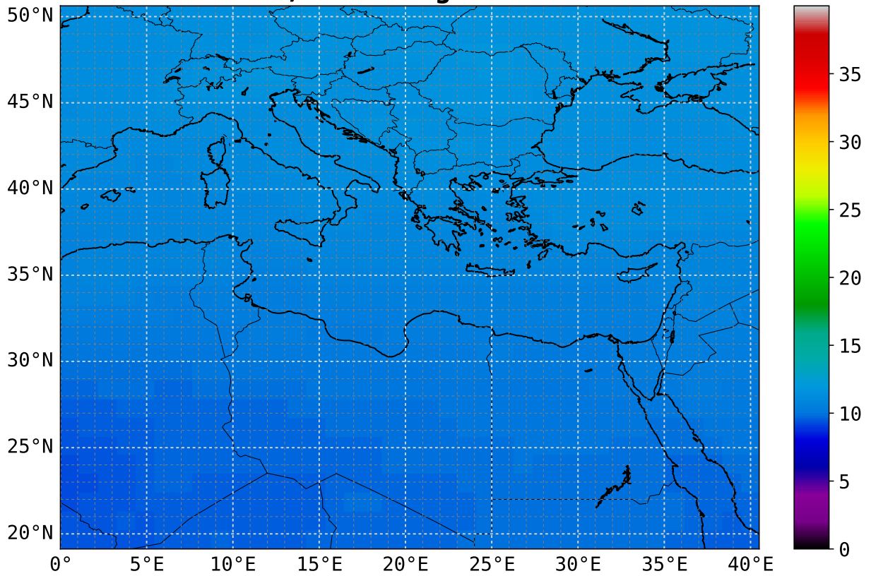
CO mean 18 UTC 7.5 km asl; scaling factor = 1e+08
