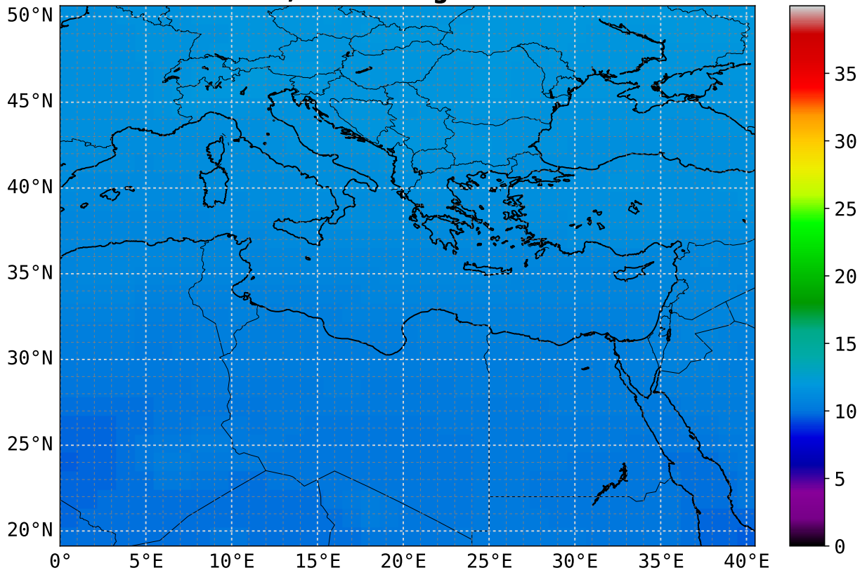
CO mean 18 UTC 6.5 km asl; scaling factor = 1e+08
