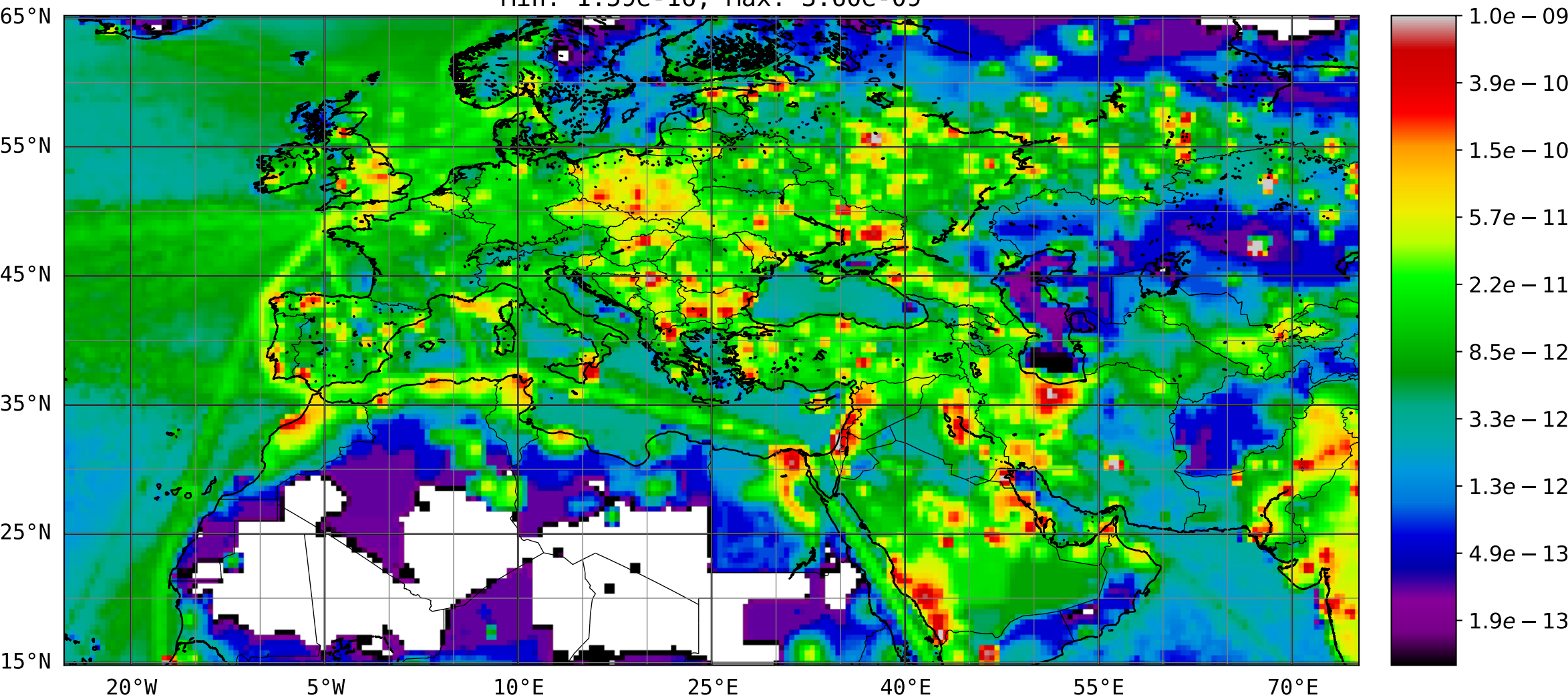
Mean of SO 2 (gas-phase precursor emis. for S04) surface flux (kgm -2 s -1 ) for period Mon, 20 Mar 2017 03Z to Mon, 01 May 2017 00Z Min: 1.59e-16; Max: 3.60e-09
