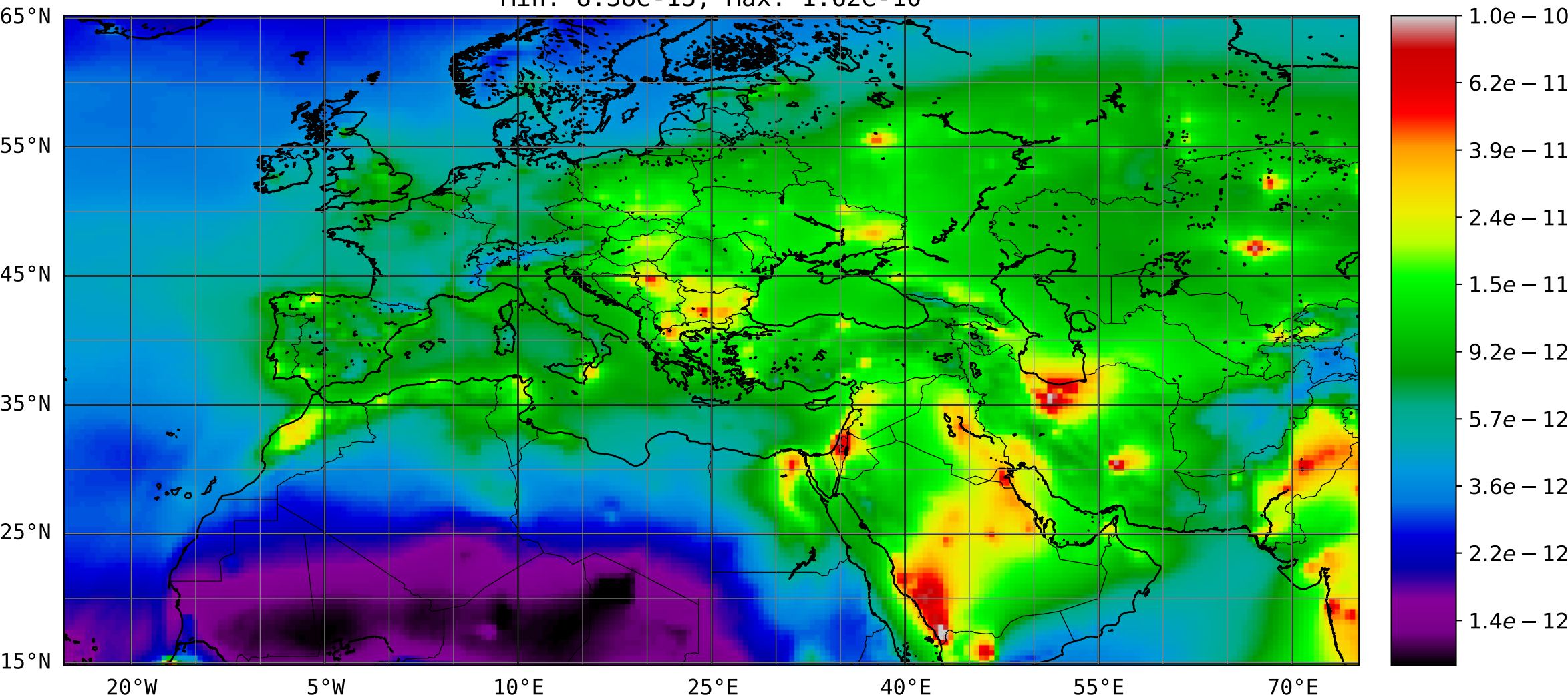
Mean of SO 4 (column-integr. prod.) surface flux ( \text{kgm}^{-2}\text{s}^{-1} ) for period Mon, 20 Mar 2017 03Z to Mon, 01 May 2017 00Z Min: 8.38\text{e-}13 ; Max: 1.62\text{e-}10
