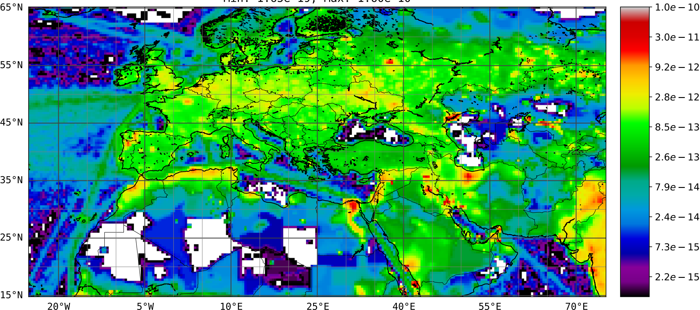
Mean of Black Carbon (hydrophobic) surface flux ( \text{kgm}^{-2}\text{s}^{-1} ) for period Mon, 20 Mar 2017 03Z to Mon, 01 May 2017 00Z Min: 1.65\text{e-}19 ; Max: 1.60\text{e-}10
