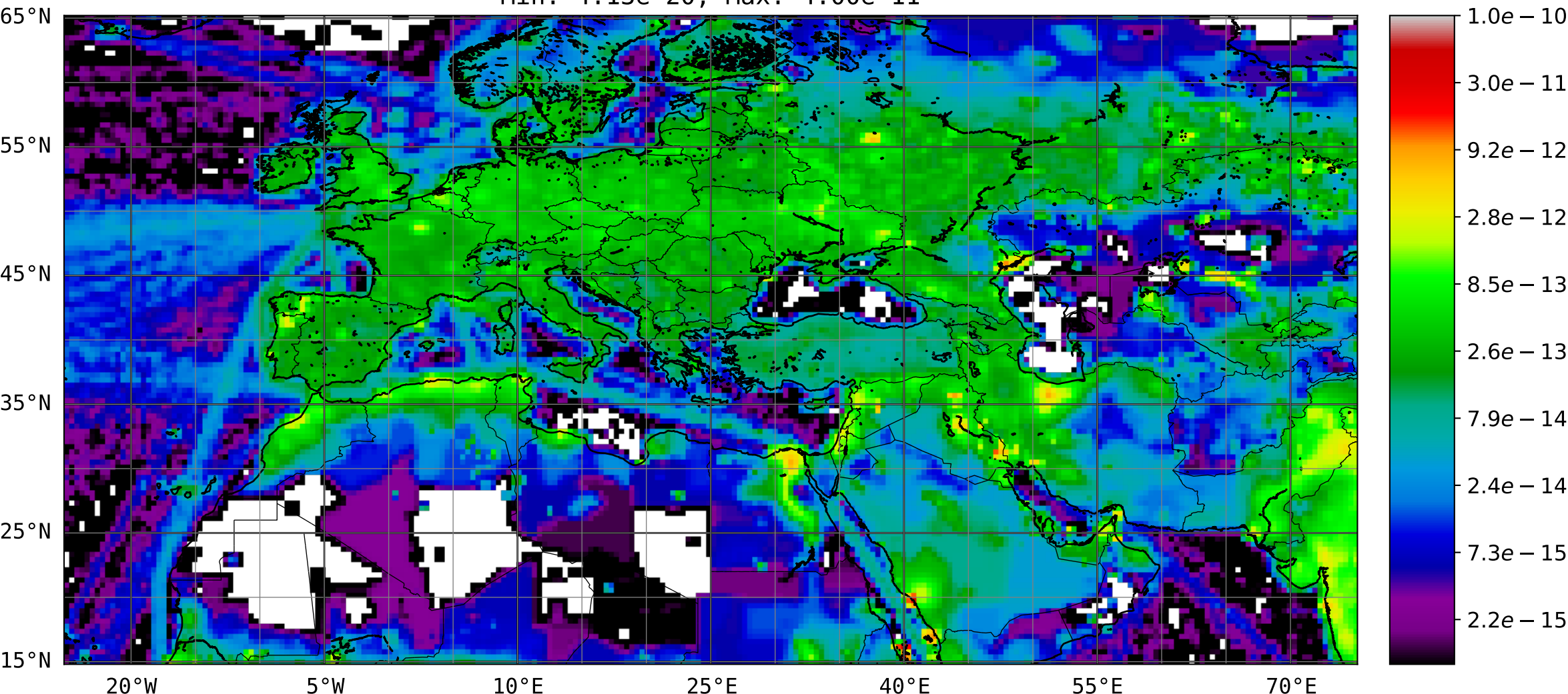
Mean of Black Carbon (hydrophilic) surface flux ( \text{kgm}^{-2}\text{s}^{-1} ) for period Mon, 20 Mar 2017 03Z to Mon, 01 May 2017 00Z Min: 4.13\text{e-}20 ; Max: 4.00\text{e-}11
