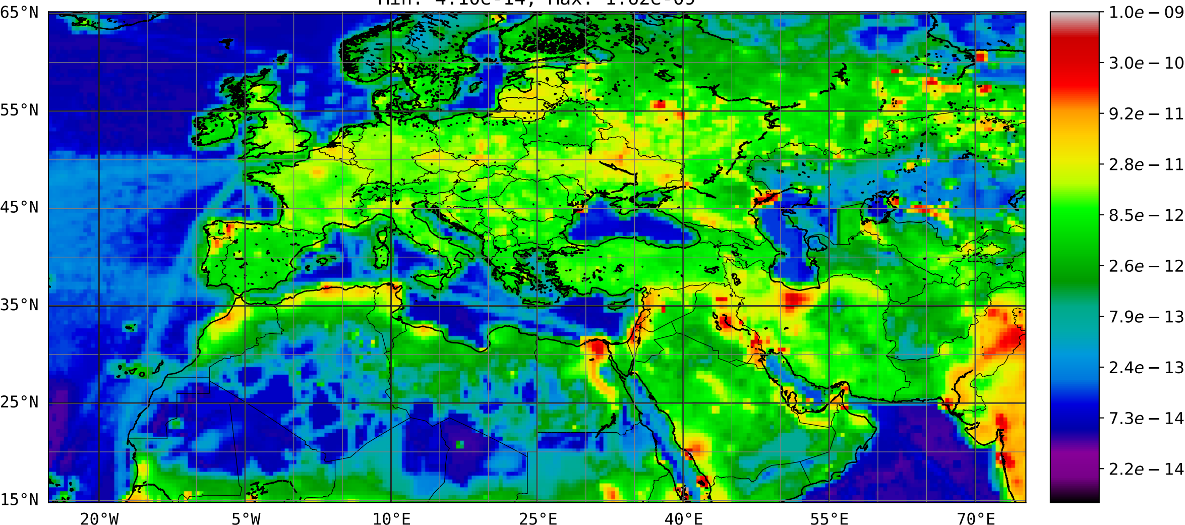
Mean of Organic Matter (hydrophilic) surface flux ( \text{kgm}^{-2}\text{s}^{-1} ) for period Mon, 20 Mar 2017 03Z to Mon, 01 May 2017 00Z Min: 4.10\text{e-}14 ; Max: 1.62\text{e-}09
