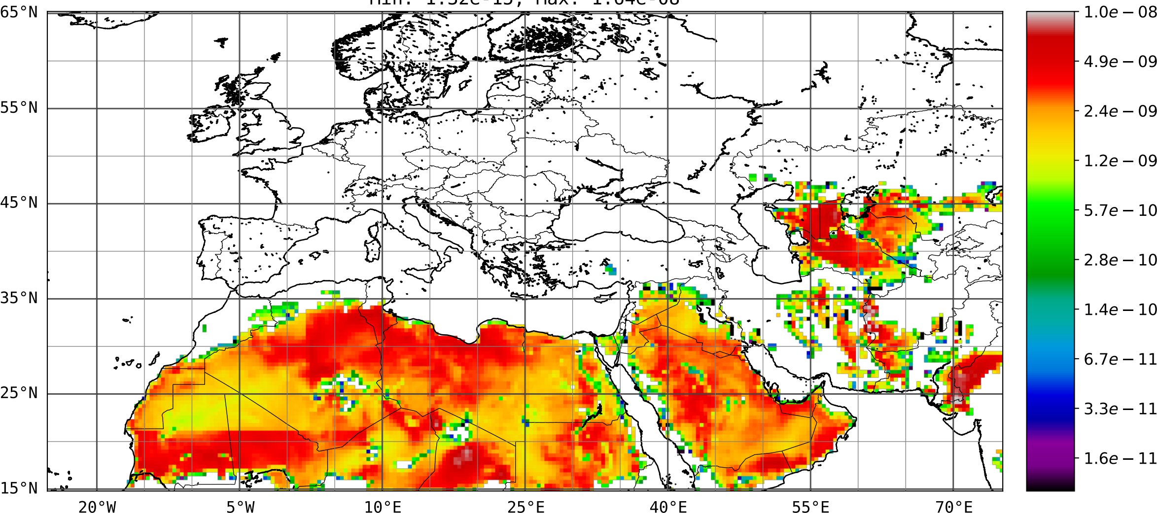
Mean of Dust (large) surface flux ( \text{kgm}^{-2}\text{s}^{-1} ) for period Mon, 20 Mar 2017 03Z to Mon, 01 May 2017 00Z Min: 1.32\text{e-}15 ; Max: 1.64\text{e-}08
