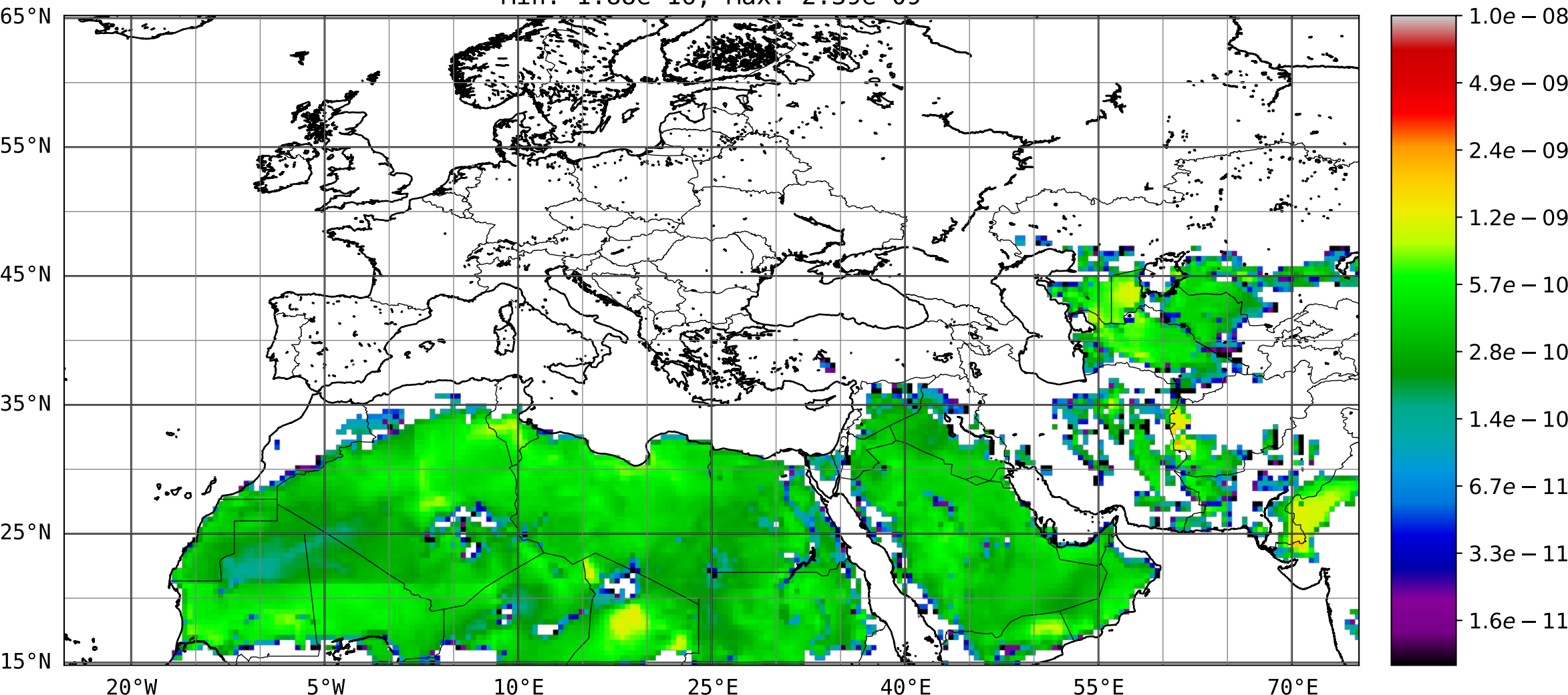
Mean of Dust (medium) surface flux ( \text{kgm}^{-2}\text{s}^{-1} ) for period Mon, 20 Mar 2017 03Z to Mon, 01 May 2017 00Z Min: 1.88\text{e-}16 ; Max: 2.39\text{e-}09
