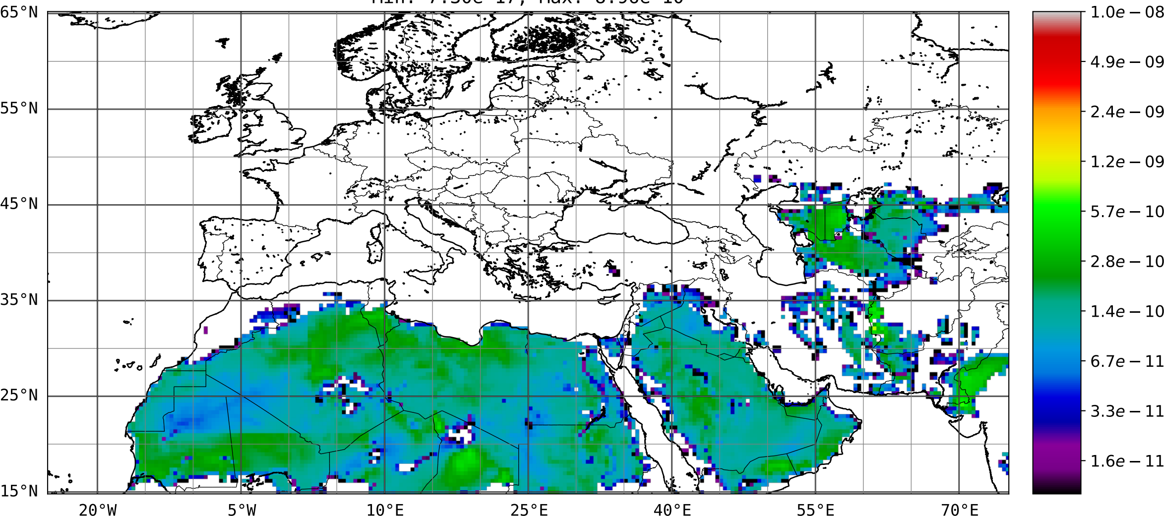
Mean of Dust (small) surface flux ( \text{kgm}^{-2}\text{s}^{-1} ) for period Mon, 20 Mar 2017 03Z to Mon, 01 May 2017 00Z Min: 7.30\text{e-}17 ; Max: 8.96\text{e-}10
